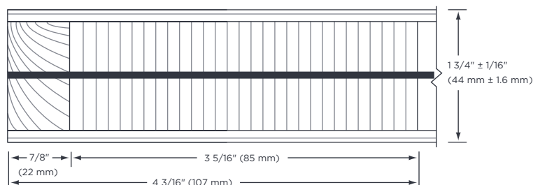
One 1/32" (0.8 mm) or 1/16" (1.6 mm) lead sheet bonded to the center of the core
